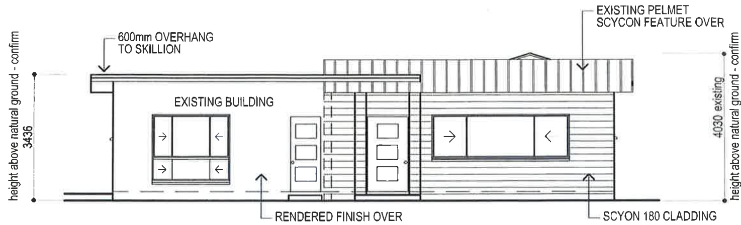
NORTH ELEVATION
