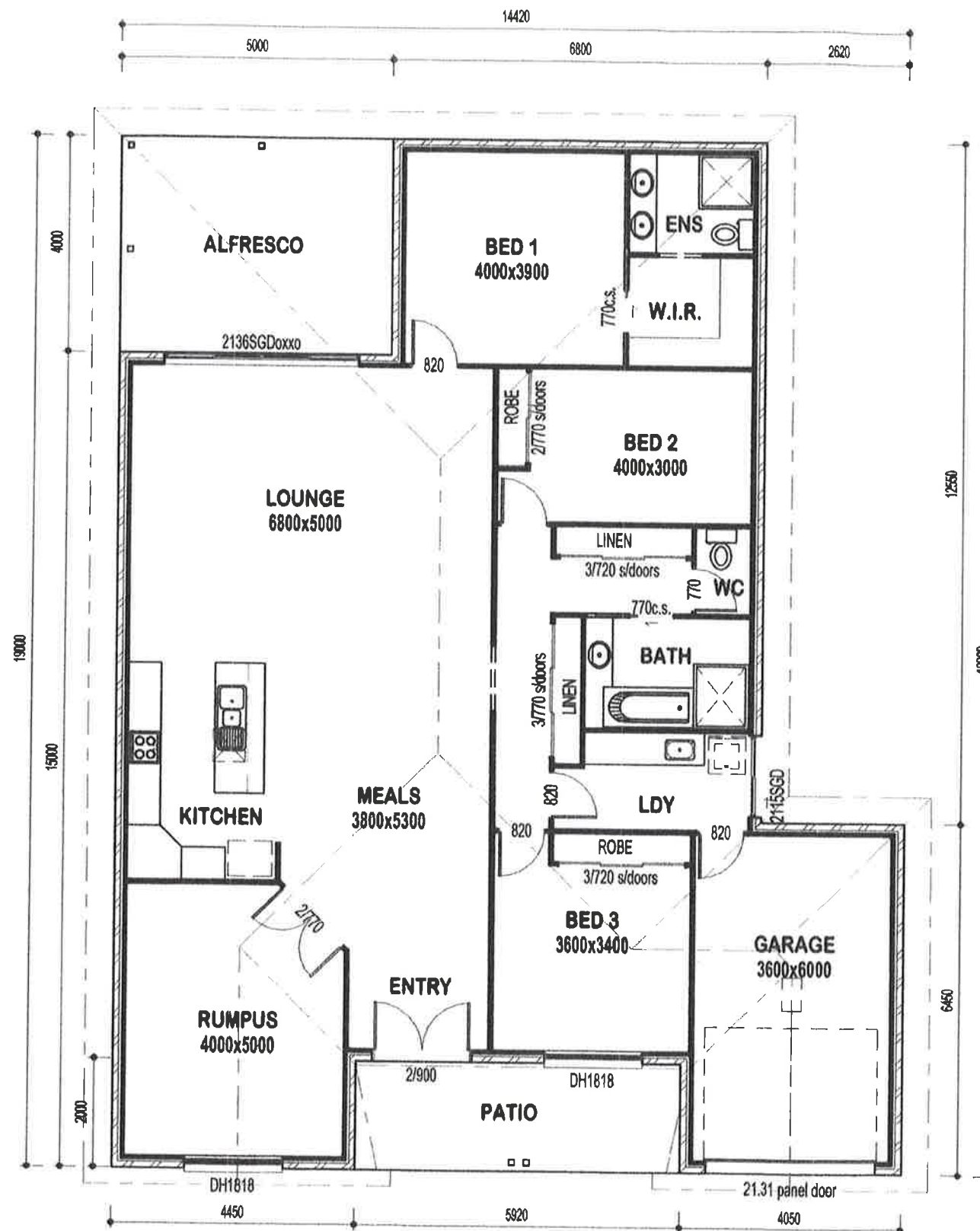
1 floor plan 1:100
