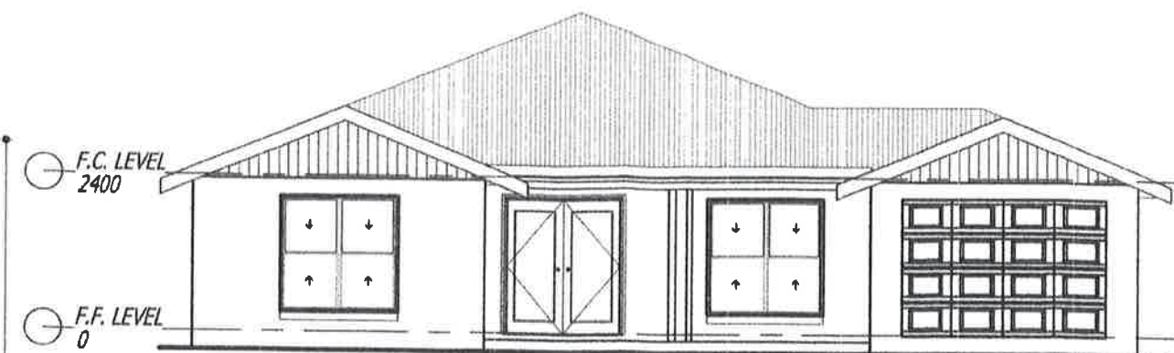
2 elevation to front 1:100
