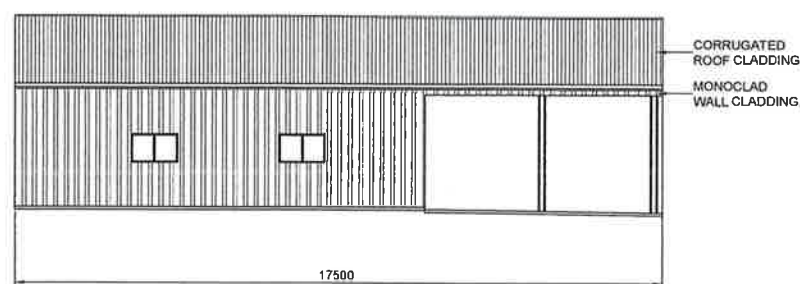
1 SIDEWALL EXTERIOR ELEVATION 6 SCALE: 1 = 200
