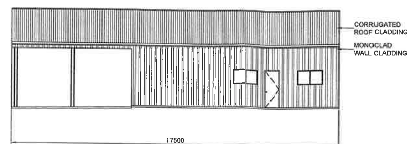
2 SIDEWALL EXTERIOR ELEVATION 6 SCALE: 1 = 200
