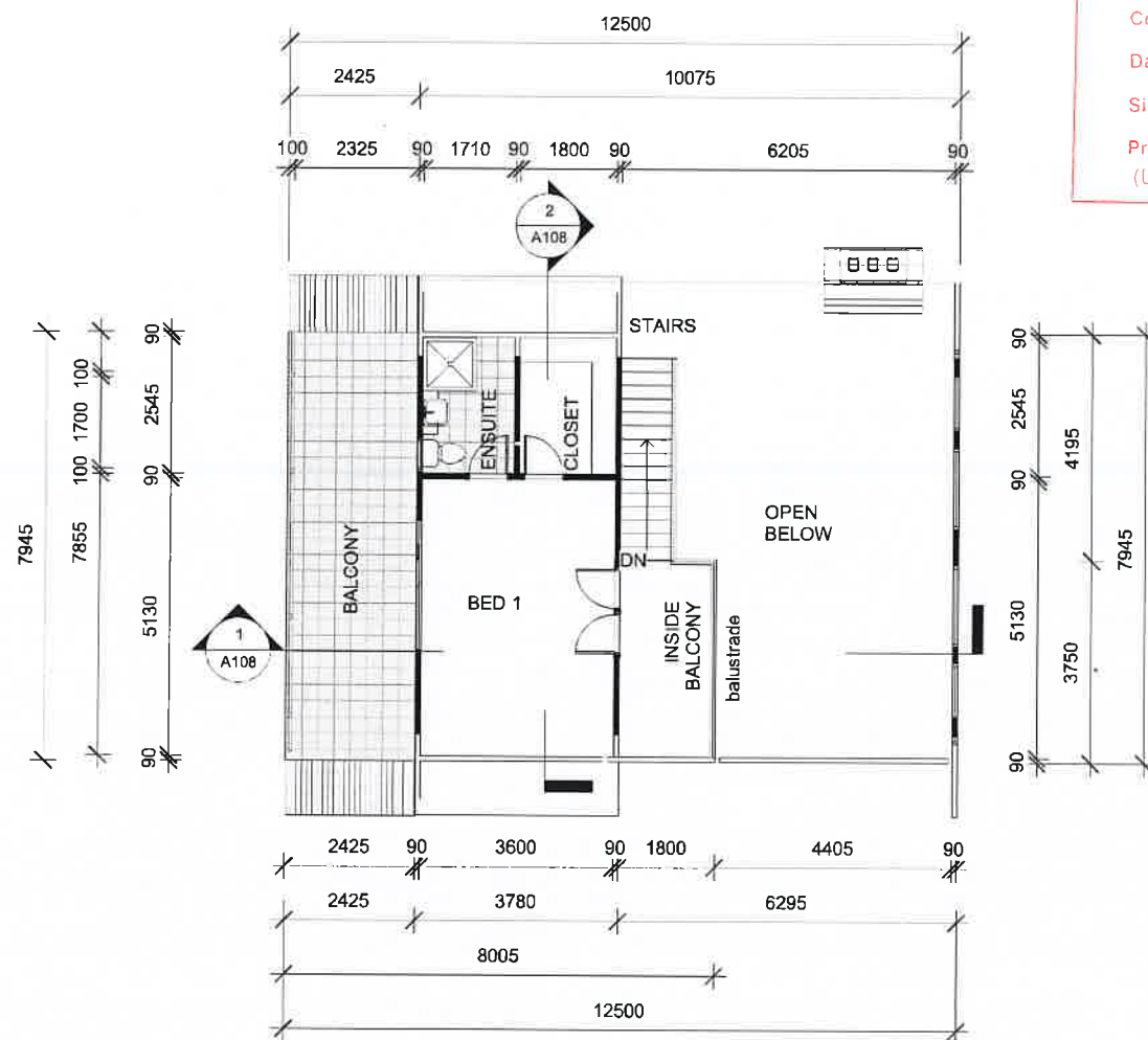
1 2nd FLOOR PLAN 1 : 100
